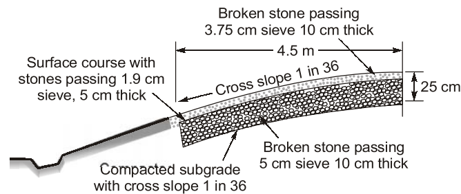
Figure-1.4: Typical cross-section of Macadam's construction
